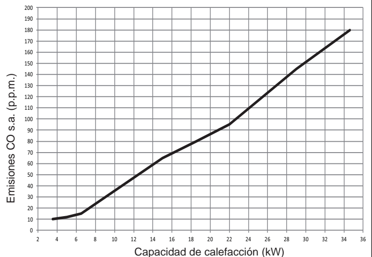
Caldera Exclusive Green HE 35 B.S.I.
