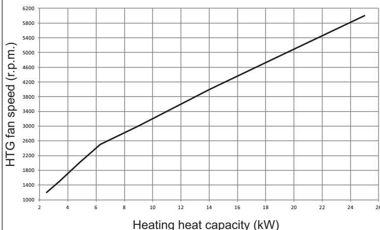
Exclusive Boiler Green HE 25 B.S.I.
