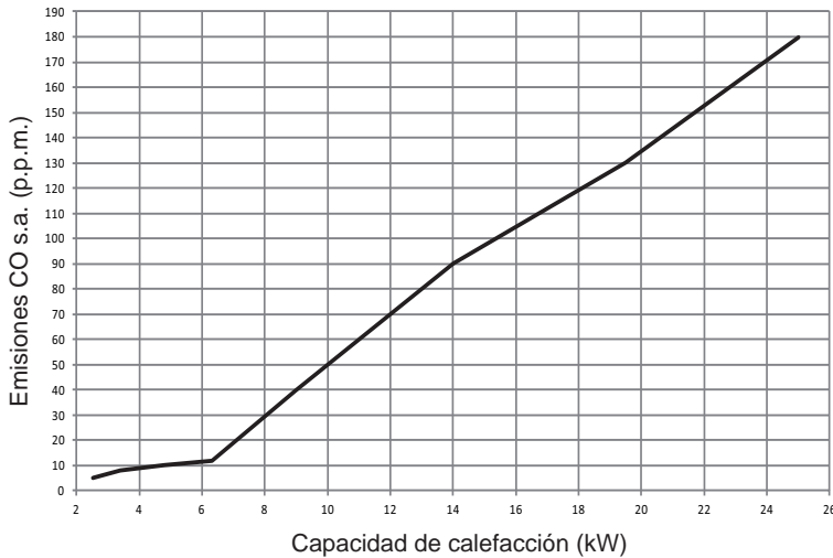
Caldera Exclusive Green HE 25 B.S.I.
